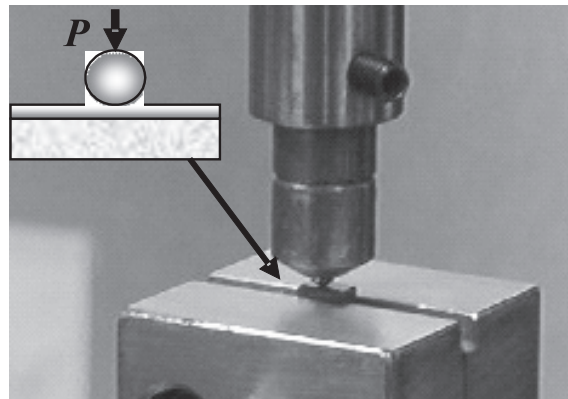
Figure 1 Mechanical set-up for the Hertzian indentation test
